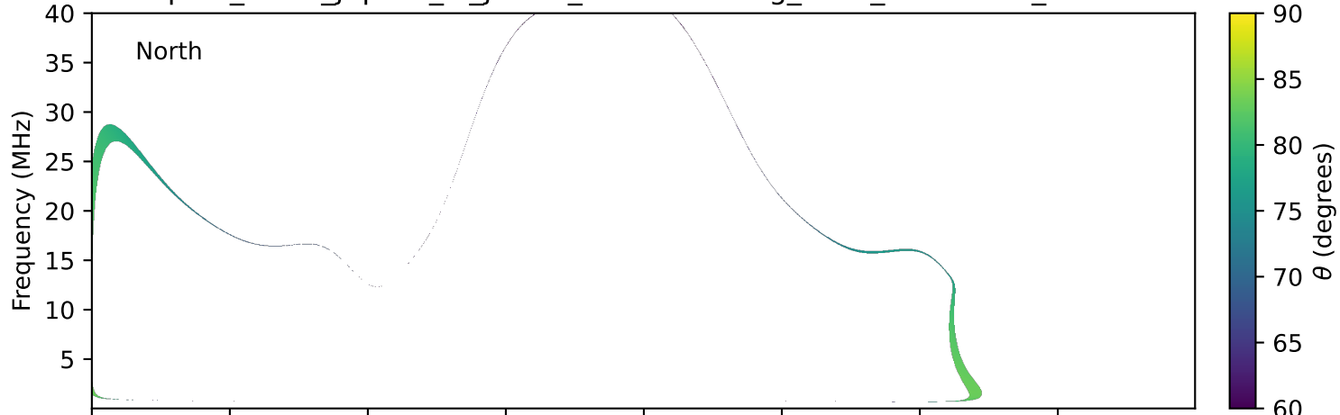
expres_earth_jupiter_io_jrm33_lossc-wid1deg_3kev_20010925_v11.cdf
