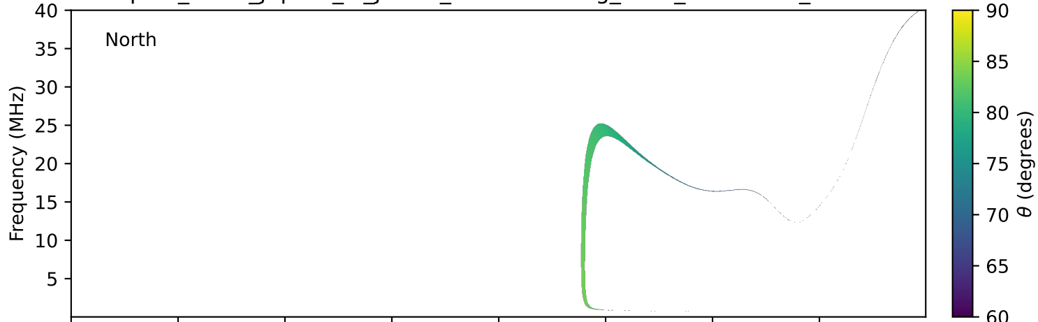
expres_earth_jupiter_io_jrm33_lossc-wid1deg_3kev_20010912_v11.cdf
