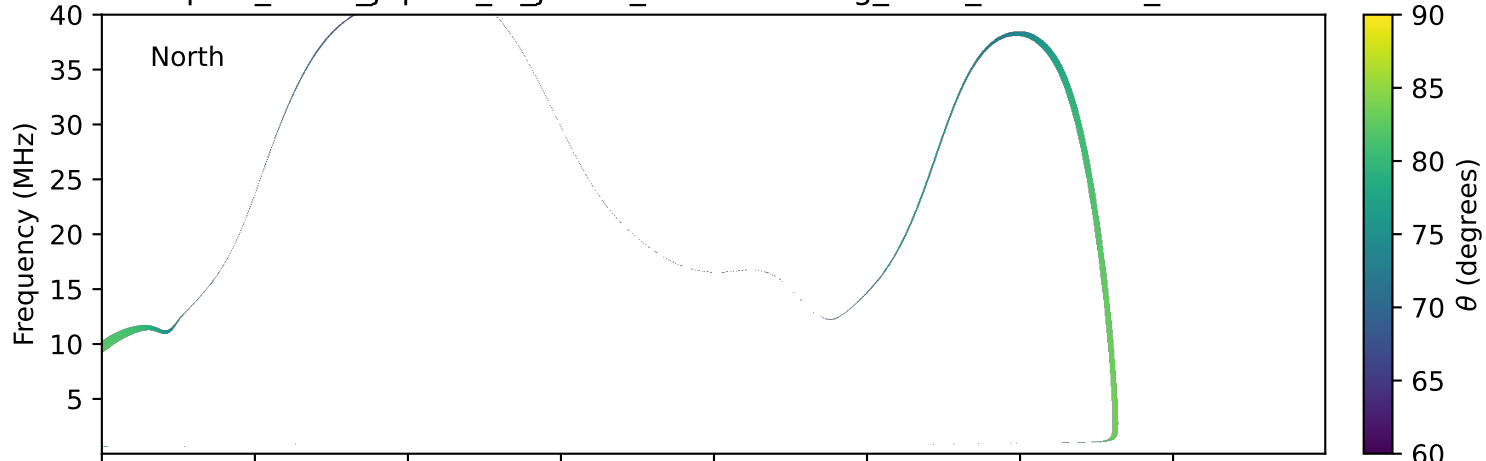
expres_earth_jupiter_io_jrm33_lossc-wid1deg_3kev_20010902_v11.cdf
