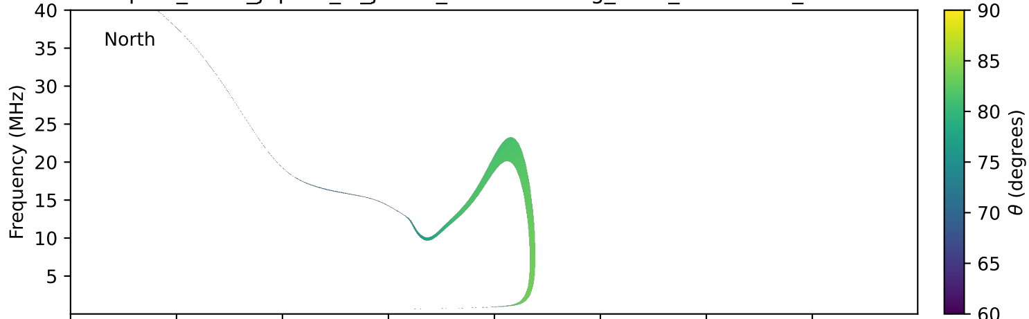
expres_earth_jupiter_io_jrm09_lossc-wid1deg_3kev_20010920_v11.cdf
