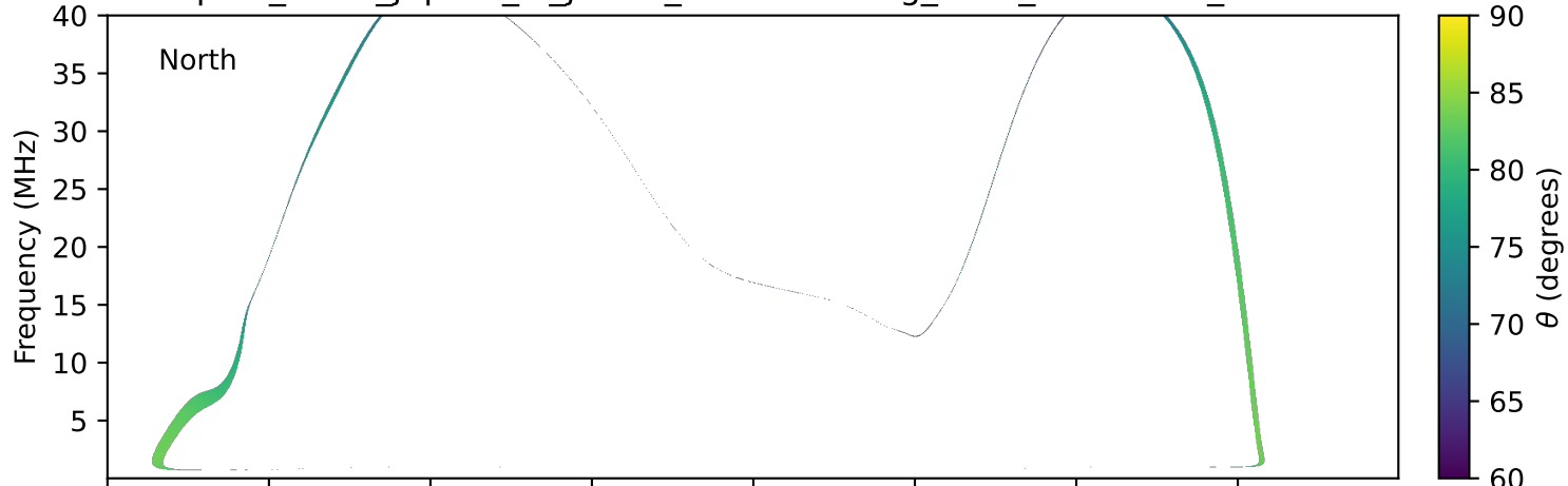
expres_earth_jupiter_io_jrm09_lossc-wid1deg_3kev_20010909_v11.cdf
