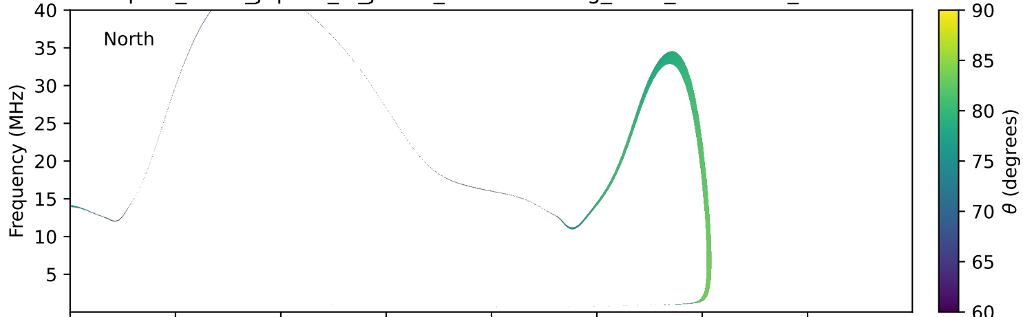
expres_earth_jupiter_io_jrm09_lossc-wid1deg_3kev_20010826_v11.cdf
