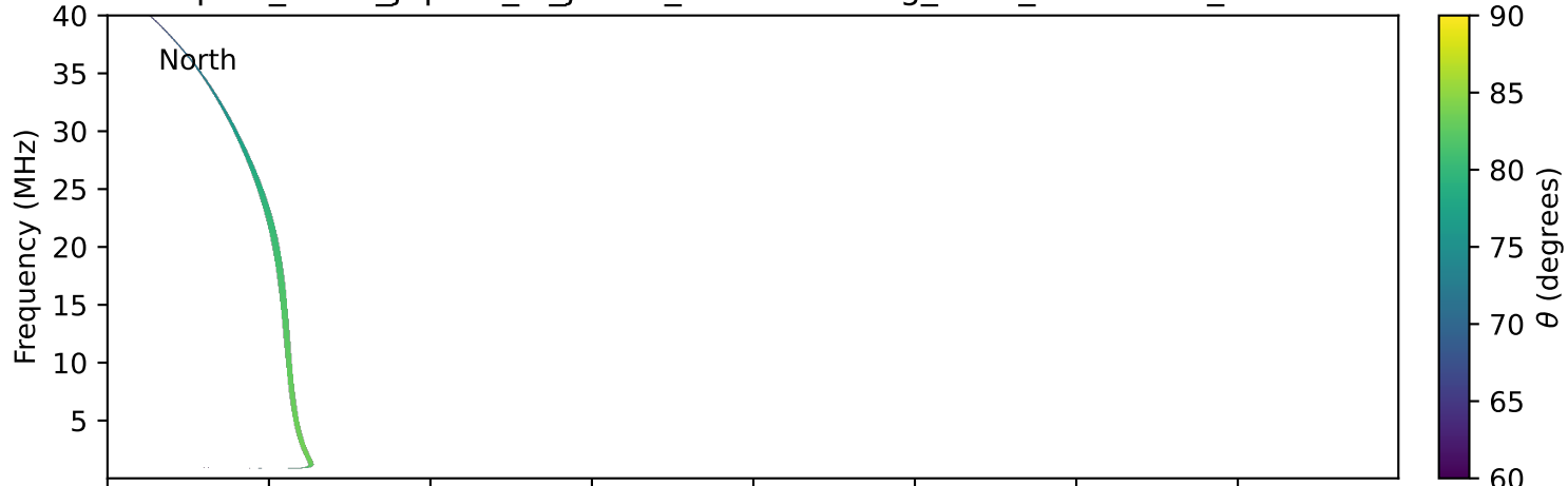
expres_earth_jupiter_io_jrm09_lossc-wid1deg_3kev_20010823_v11.cdf
