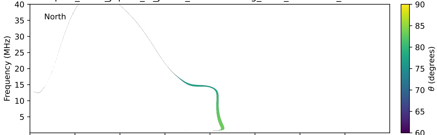
expres_earth_jupiter_io_jrm09_lossc-wid1deg_3kev_20010812_v11.cdf
