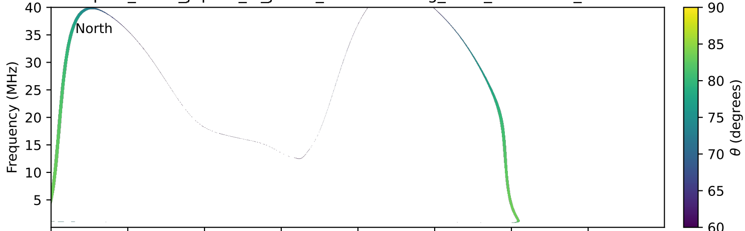
expres_earth_jupiter_io_jrm09_lossc-wid1deg_3kev_20010810_v11.cdf
