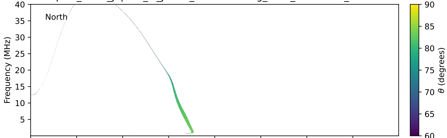
expres_earth_jupiter_io_jrm09_lossc-wid1deg_3kev_20010805_v11.cdf
