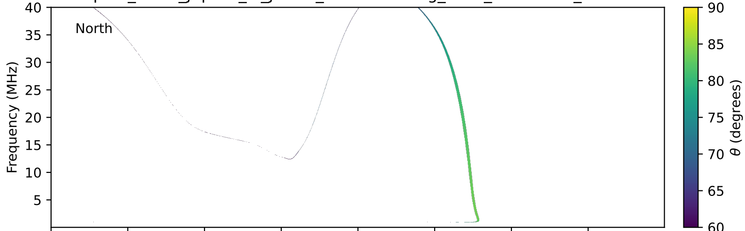
expres_earth_jupiter_io_jrm09_lossc-wid1deg_3kev_20010803_v11.cdf
