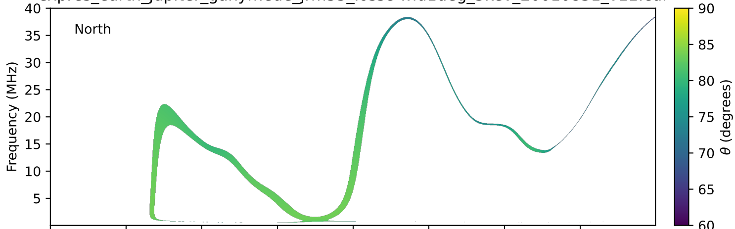
expres_earth_jupiter_ganymede_jrm33_lossc-wid1deg_3kev_20010831_v11.cdf
