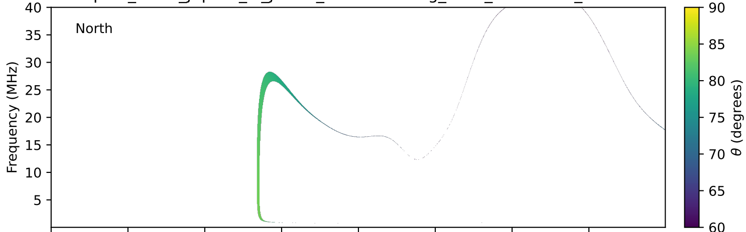
expres_earth_jupiter_io_jrm33_lossc-wid1deg_3kev_20010730_v11.cdf
