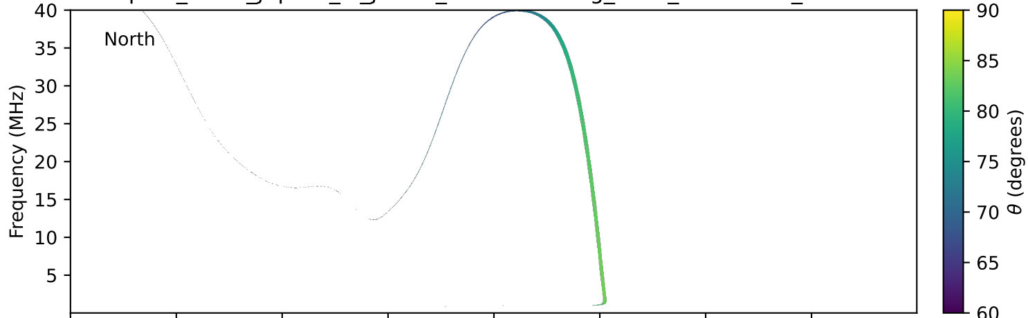
expres_earth_jupiter_io_jrm33_lossc-wid1deg_3kev_20010727_v11.cdf
