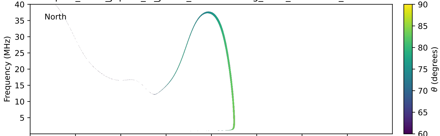
expres_earth_jupiter_io_jrm33_lossc-wid1deg_3kev_20010720_v11.cdf
