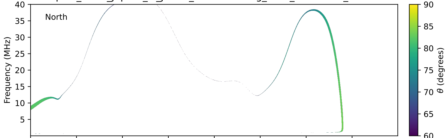
expres_earth_jupiter_io_jrm33_lossc-wid1deg_3kev_20010716_v11.cdf
