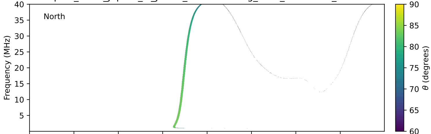
expres_earth_jupiter_io_jrm33_lossc-wid1deg_3kev_20010705_v11.cdf
