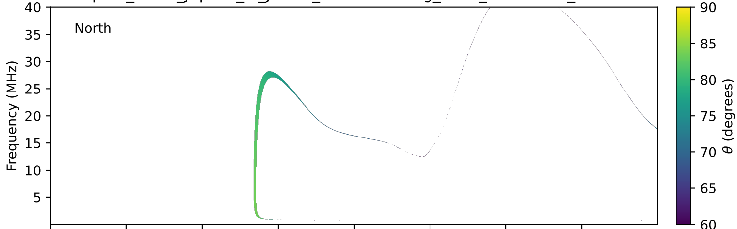
expres_earth_jupiter_io_jrm09_lossc-wid1deg_3kev_20010730_v11.cdf
