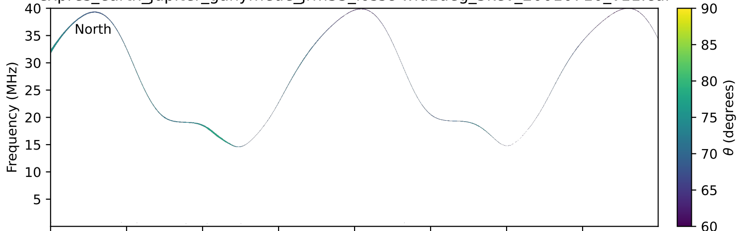
expres_earth_jupiter_ganymede_jrm33_lossc-wid1deg_3kev_20010710_v11.cdf
