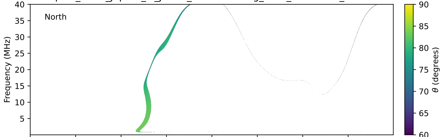
expres_earth_jupiter_io_jrm33_lossc-wid1deg_3kev_20010628_v11.cdf
