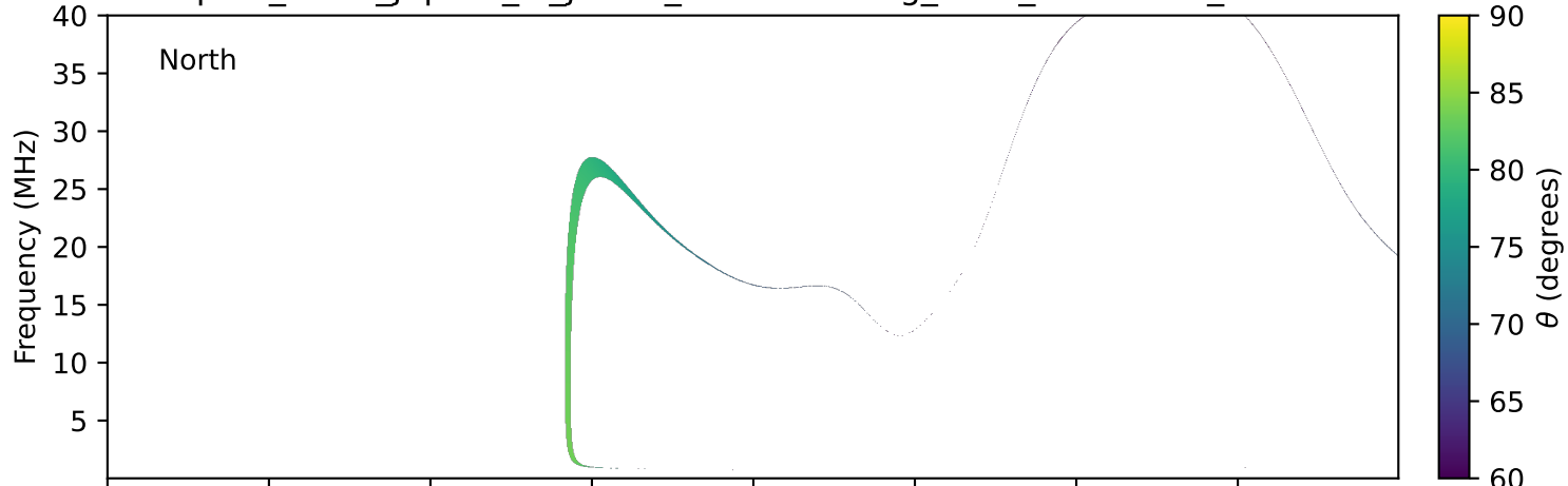
expres_earth_jupiter_io_jrm33_lossc-wid1deg_3kev_20010612_v11.cdf
