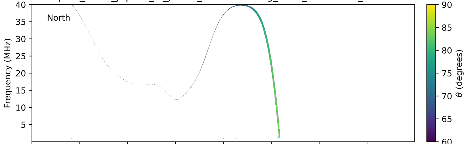
expres_earth_jupiter_io_jrm33_lossc-wid1deg_3kev_20010609_v11.cdf
