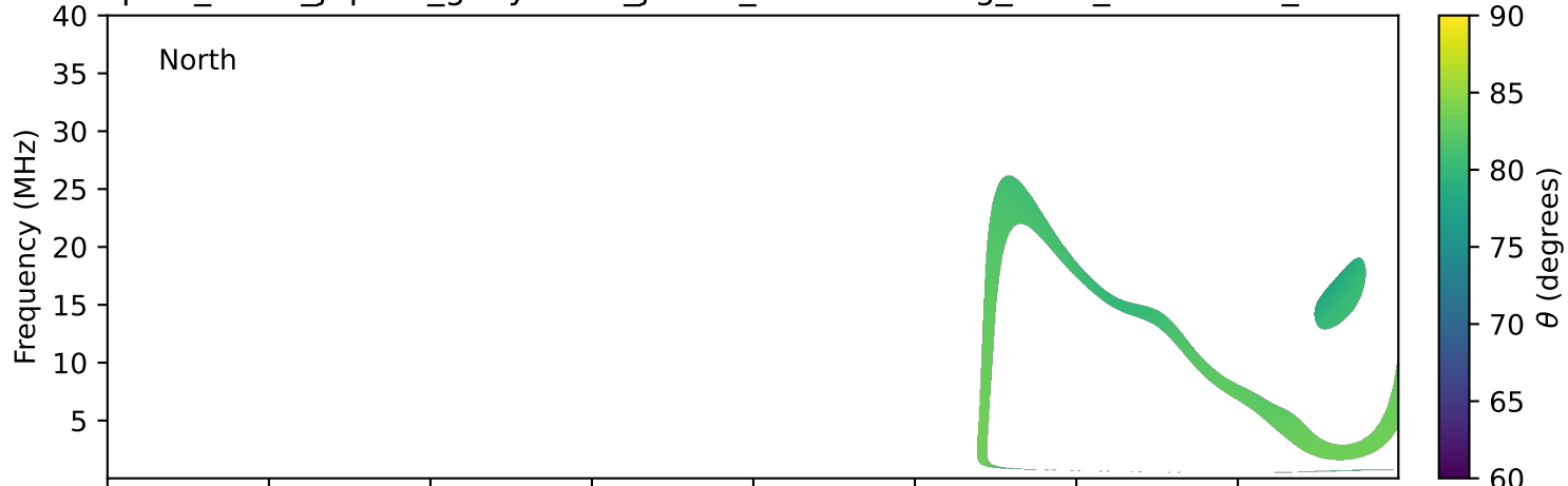
expres_earth_jupiter_ganymede_jrm33_lossc-wid1deg_3kev_20010610_v11.cdf
