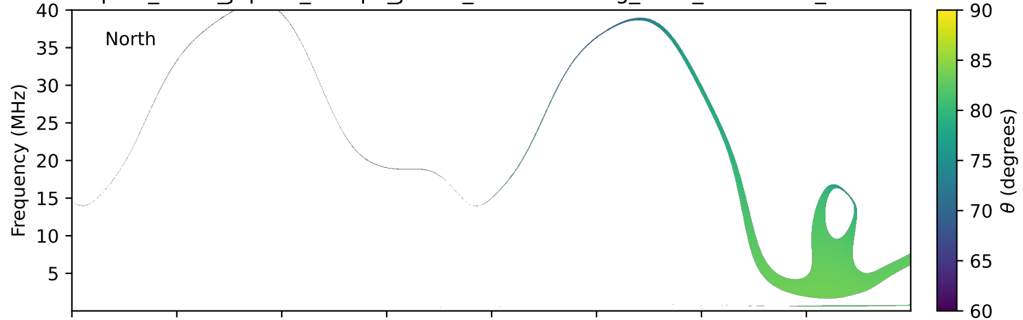
expres_earth_jupiter_europa_jrm33_lossc-wid1deg_3kev_20010606_v11.cdf
