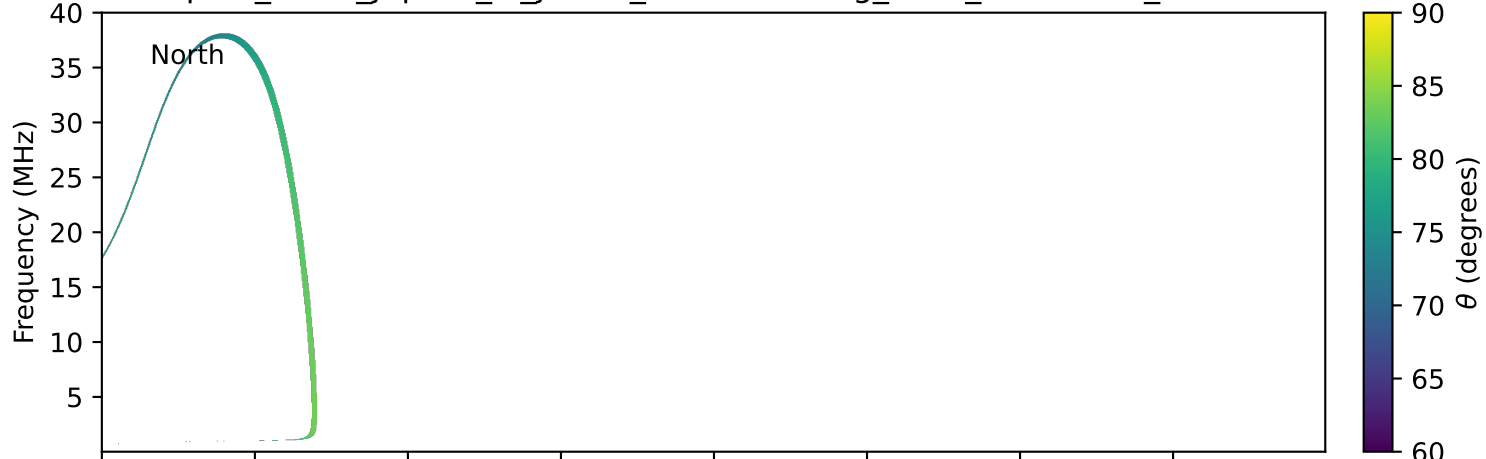
expres_earth_jupiter_io_jrm33_lossc-wid1deg_3kev_20010521_v11.cdf
