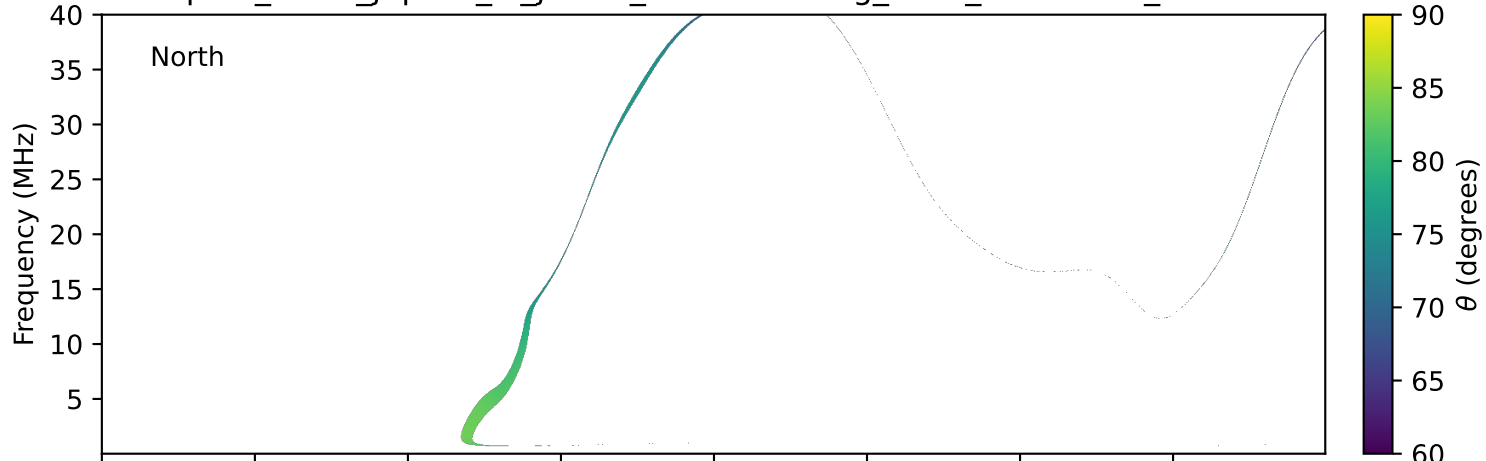
expres_earth_jupiter_io_jrm33_lossc-wid1deg_3kev_20010506_v11.cdf
