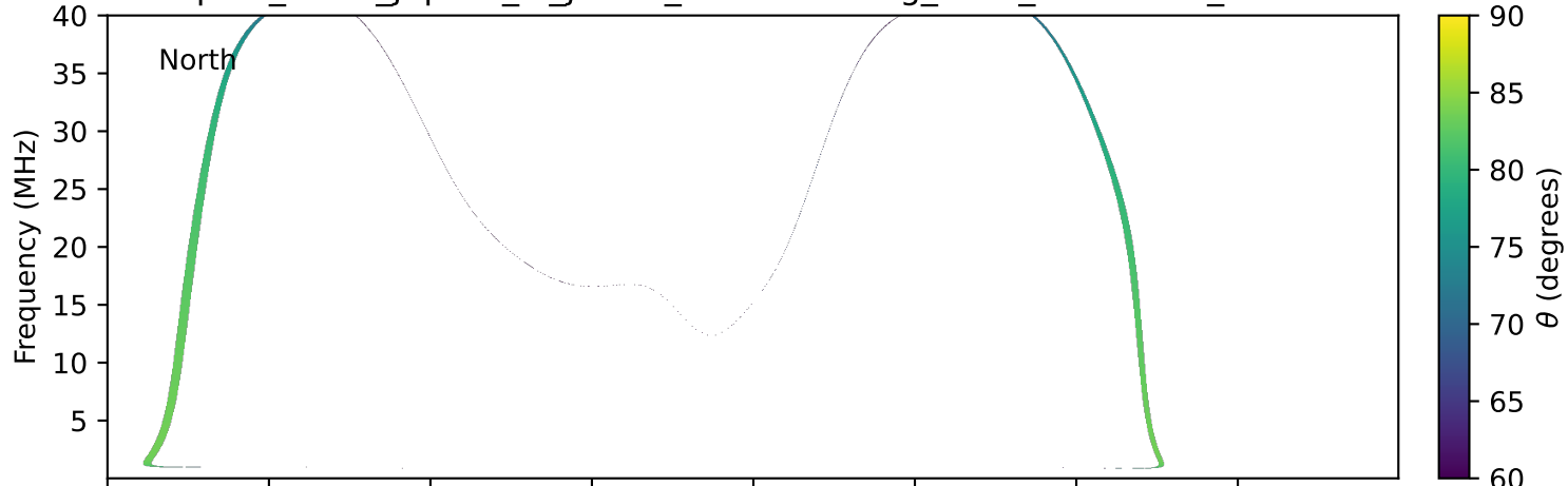
expres_earth_jupiter_io_jrm33_lossc-wid1deg_3kev_20010501_v11.cdf
