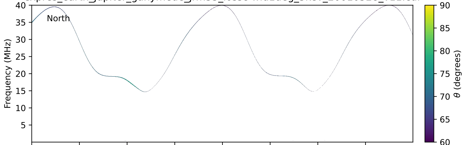
expres_earth_jupiter_ganymede_jrm33_lossc-wid1deg_3kev_20010528_v11.cdf
