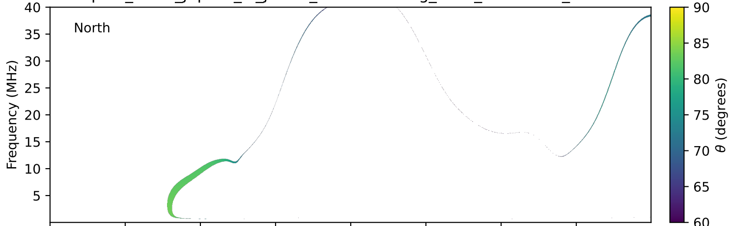
expres_earth_jupiter_io_jrm33_lossc-wid1deg_3kev_20010429_v11.cdf
