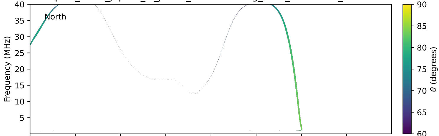
expres_earth_jupiter_io_jrm33_lossc-wid1deg_3kev_20010424_v11.cdf
