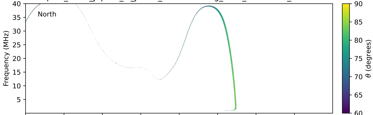
expres_earth_jupiter_io_jrm33_lossc-wid1deg_3kev_20010417_v11.cdf
