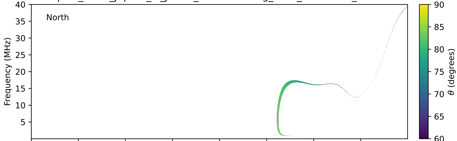
expres_earth_jupiter_io_jrm33_lossc-wid1deg_3kev_20010402_v11.cdf
