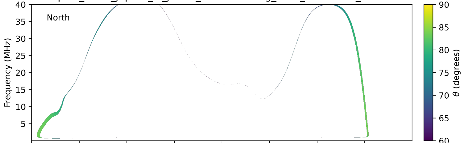
expres_earth_jupiter_io_jrm33_lossc-wid1deg_3kev_20010323_v11.cdf
