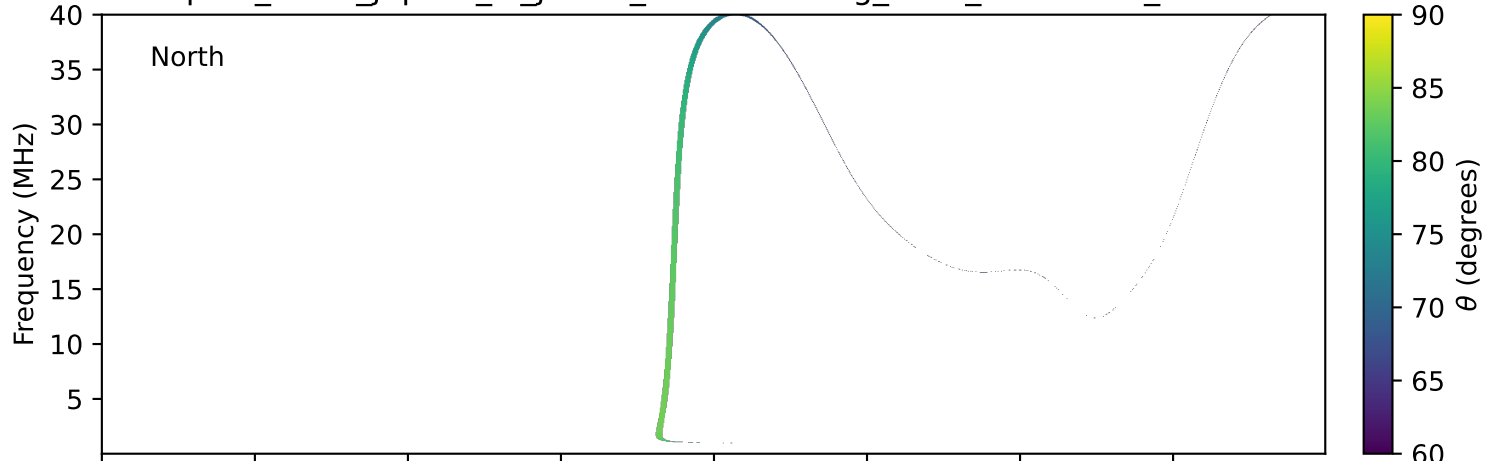
expres_earth_jupiter_io_jrm33_lossc-wid1deg_3kev_20010312_v11.cdf
