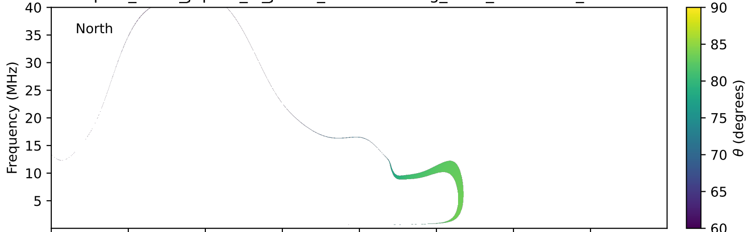
expres_earth_jupiter_io_jrm33_lossc-wid1deg_3kev_20010302_v11.cdf
