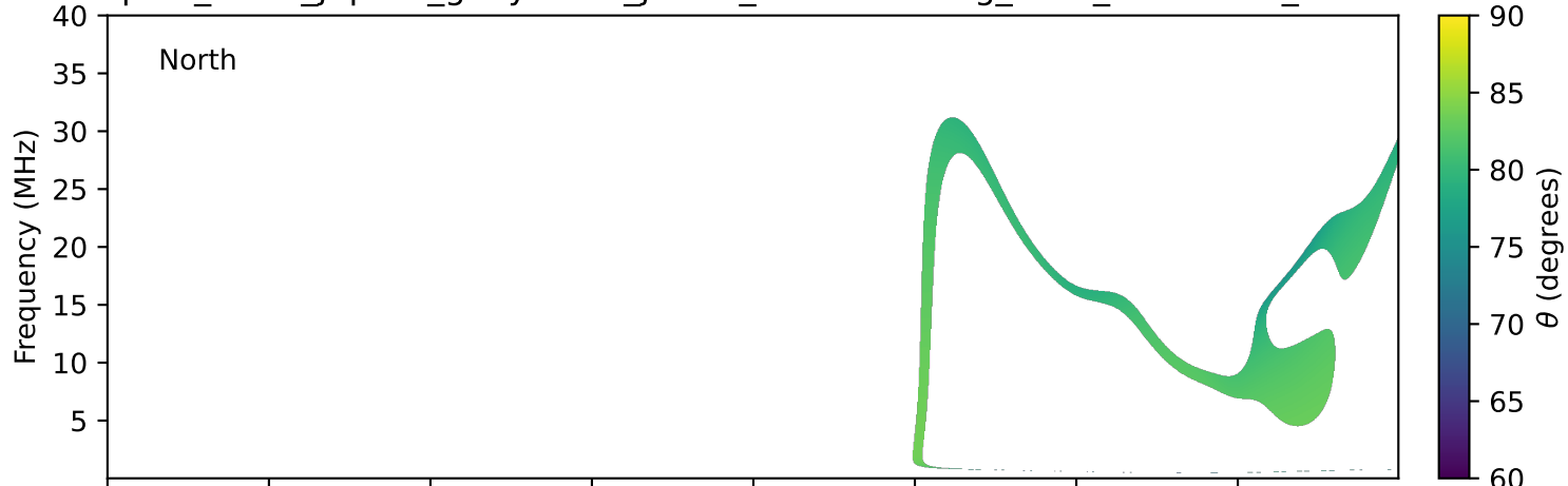
expres_earth_jupiter_ganymede_jrm33_lossc-wid1deg_3kev_20010304_v11.cdf
