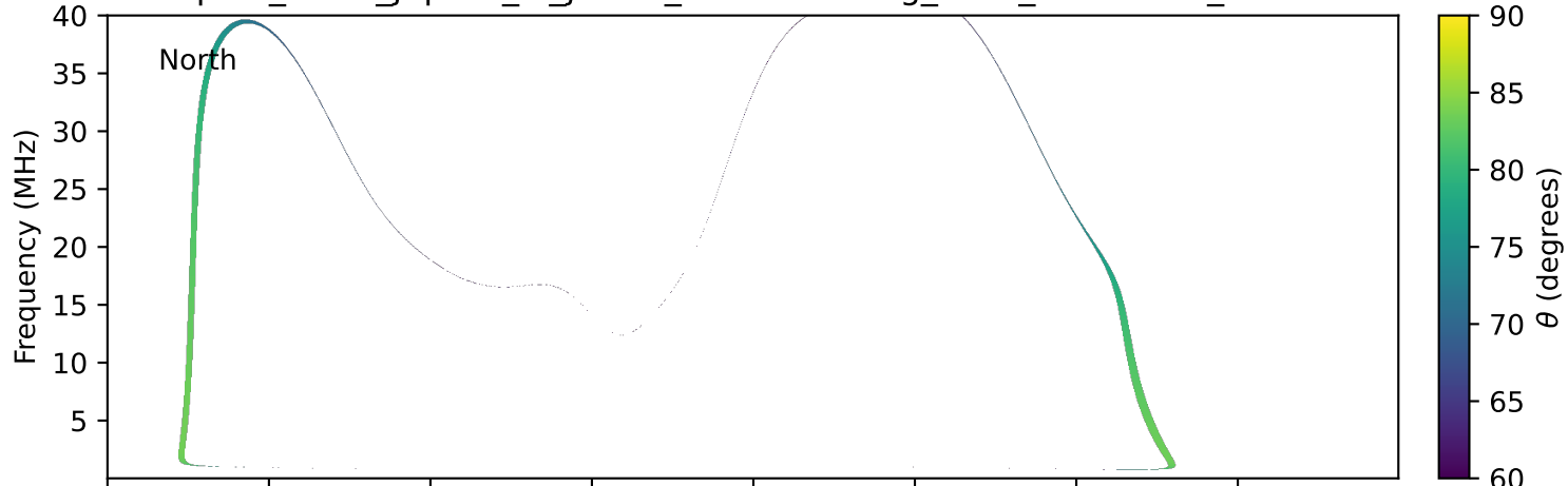
expres_earth_jupiter_io_jrm33_lossc-wid1deg_3kev_20010228_v11.cdf
