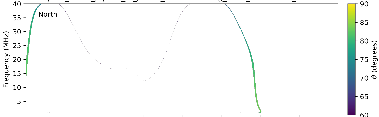
expres_earth_jupiter_io_jrm33_lossc-wid1deg_3kev_20010221_v11.cdf
