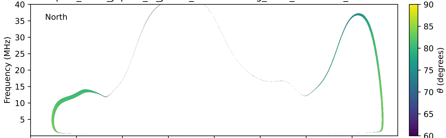
expres_earth_jupiter_io_jrm33_lossc-wid1deg_3kev_20010212_v11.cdf
