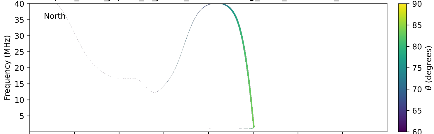
expres_earth_jupiter_io_jrm33_lossc-wid1deg_3kev_20010207_v11.cdf
