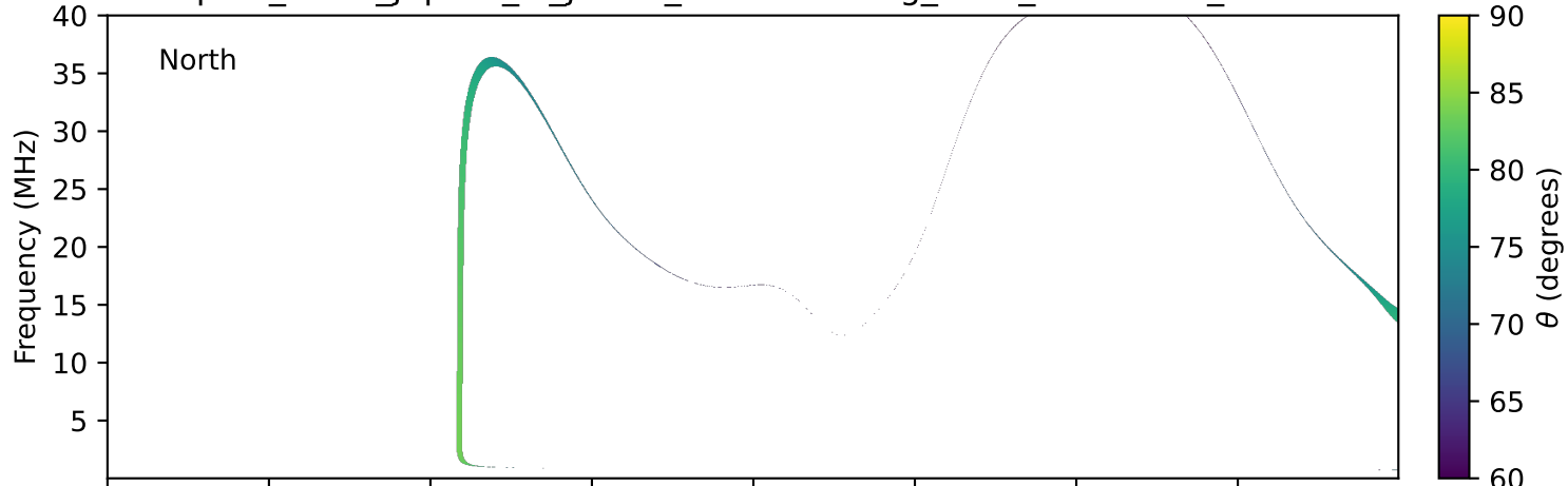
expres_earth_jupiter_io_jrm33_lossc-wid1deg_3kev_20010203_v11.cdf
