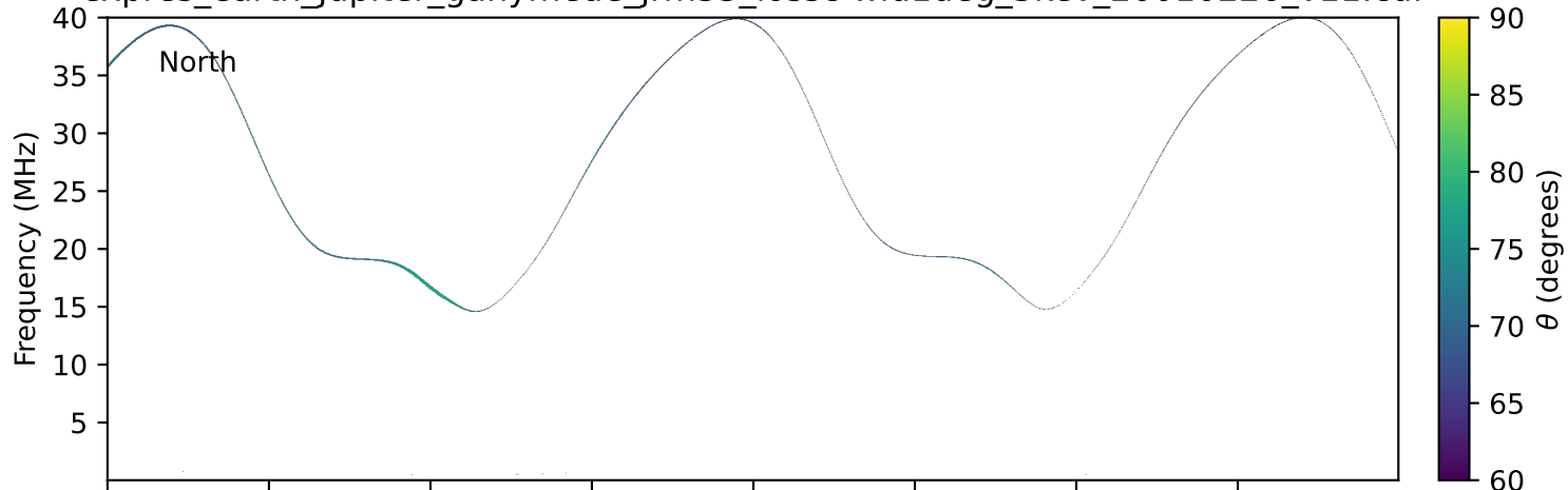
expres_earth_jupiter_ganymede_jrm33_lossc-wid1deg_3kev_20010226_v11.cdf
