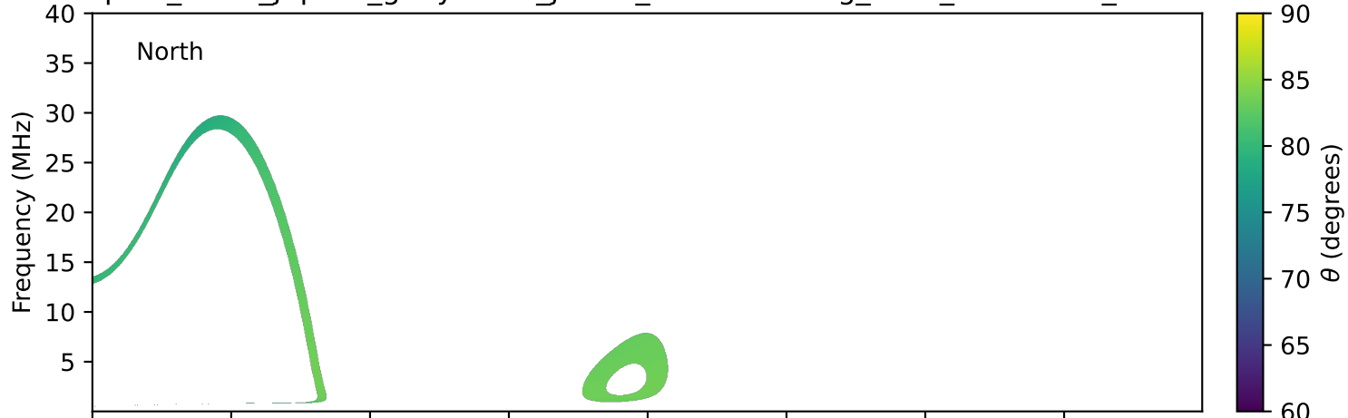
expres_earth_jupiter_ganymede_jrm33_lossc-wid1deg_3kev_20010207_v11.cdf
