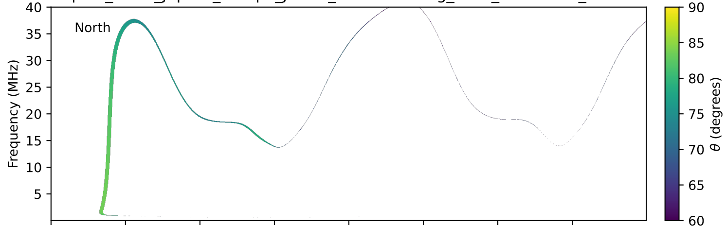
expres_earth_jupiter_europa_jrm33_lossc-wid1deg_3kev_20010223_v11.cdf
