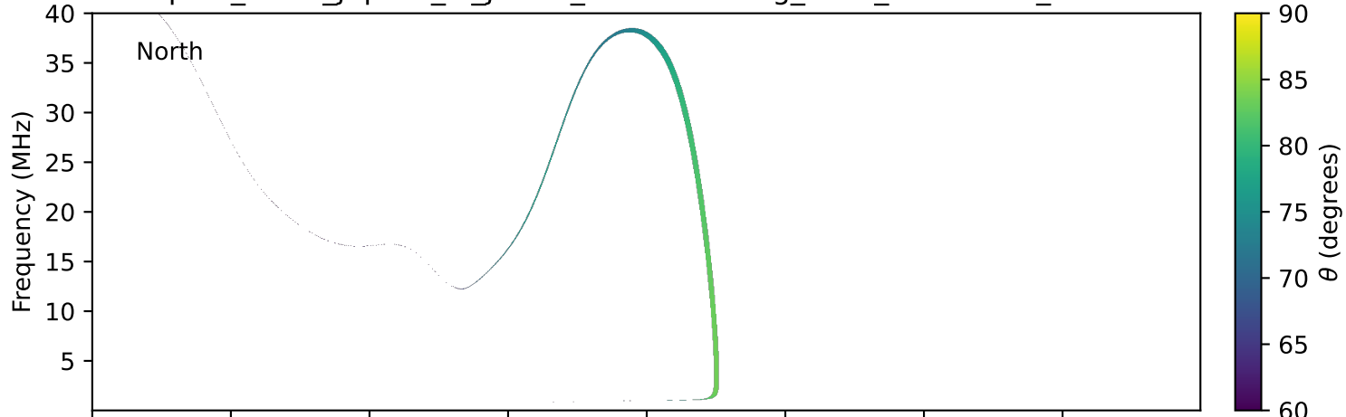
expres_earth_jupiter_io_jrm33_lossc-wid1deg_3kev_20010131_v11.cdf
