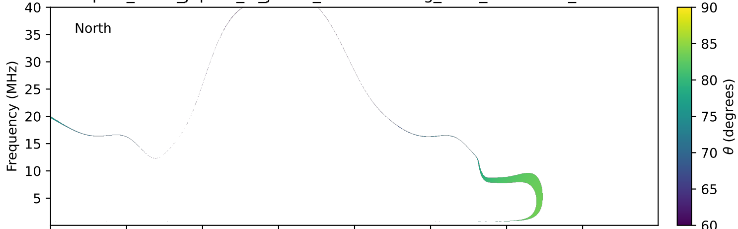
expres_earth_jupiter_io_jrm33_lossc-wid1deg_3kev_20010129_v11.cdf
