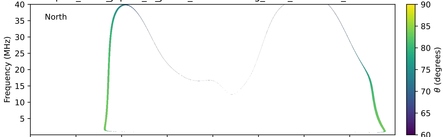
expres_earth_jupiter_io_jrm33_lossc-wid1deg_3kev_20010127_v11.cdf
