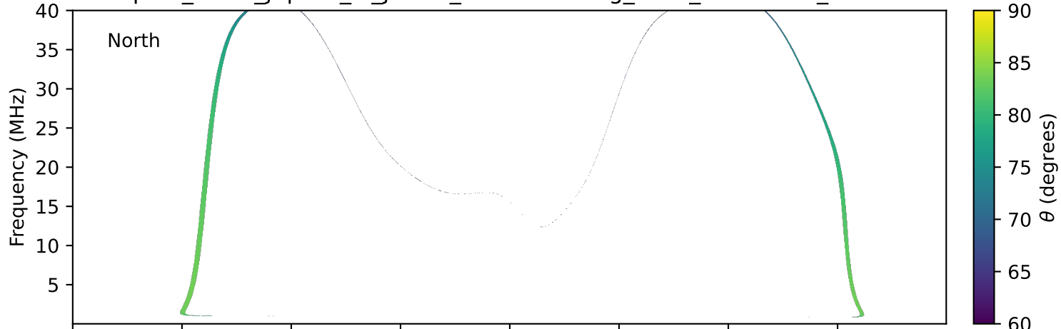
expres_earth_jupiter_io_jrm33_lossc-wid1deg_3kev_20010120_v11.cdf
