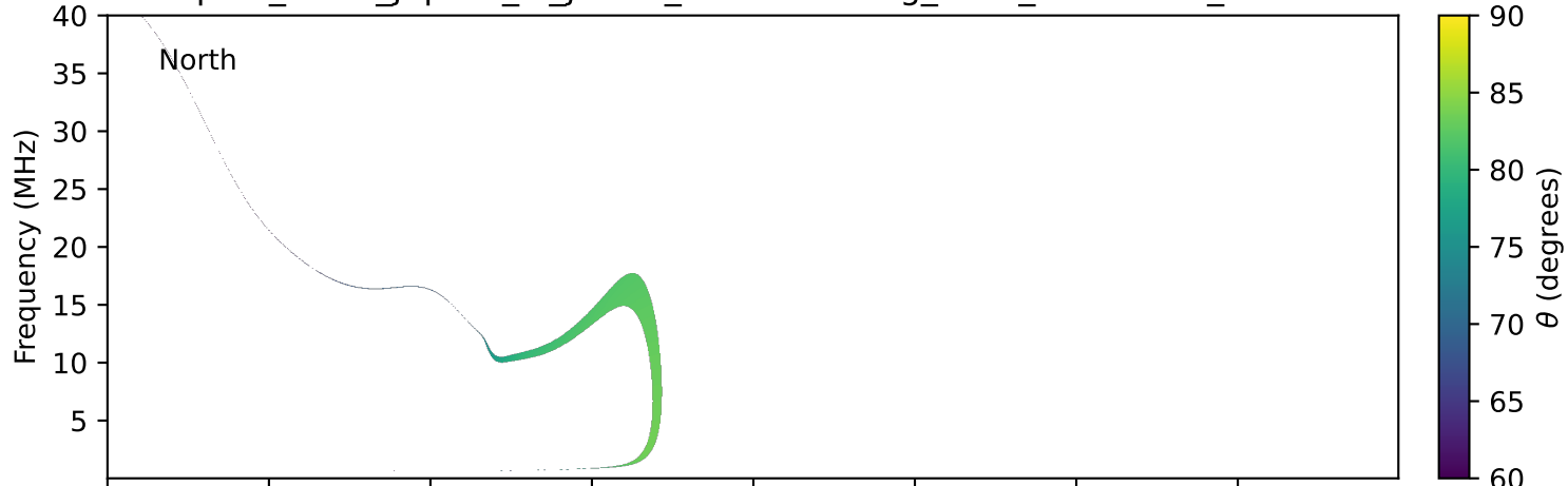
expres_earth_jupiter_io_jrm33_lossc-wid1deg_3kev_20010117_v11.cdf
