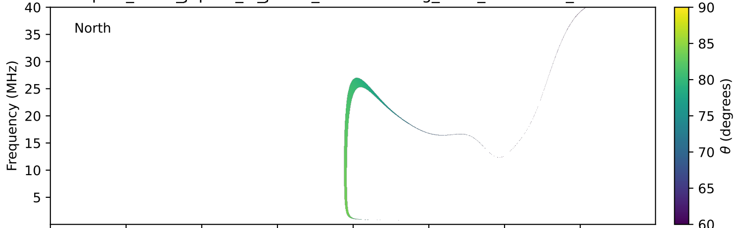
expres_earth_jupiter_io_jrm33_lossc-wid1deg_3kev_20010109_v11.cdf
